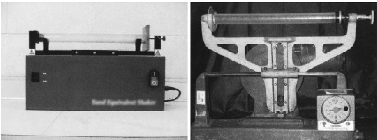
FIG. 2 Mechanized Shakers
